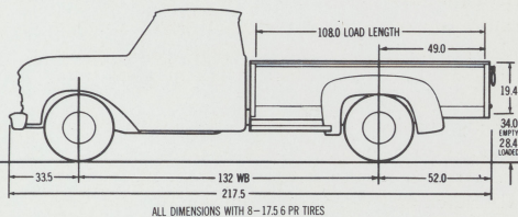
PICKUP BODY DIMENSIONS
